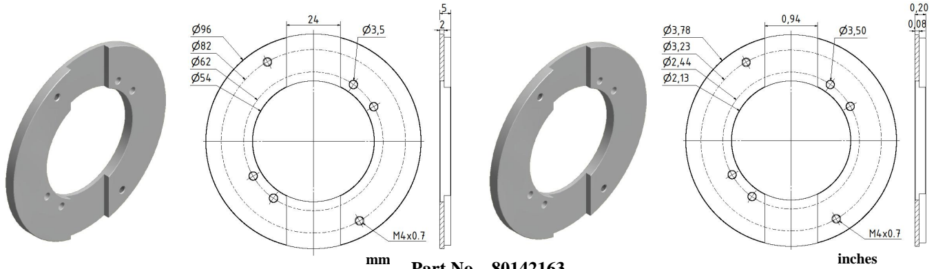
mm Part No. 80142163 Material: Aluminium
