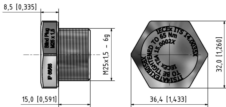
Blind Plug - Type 25
