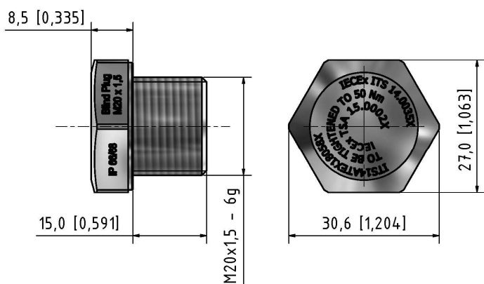
Blind Plug - Type 20
